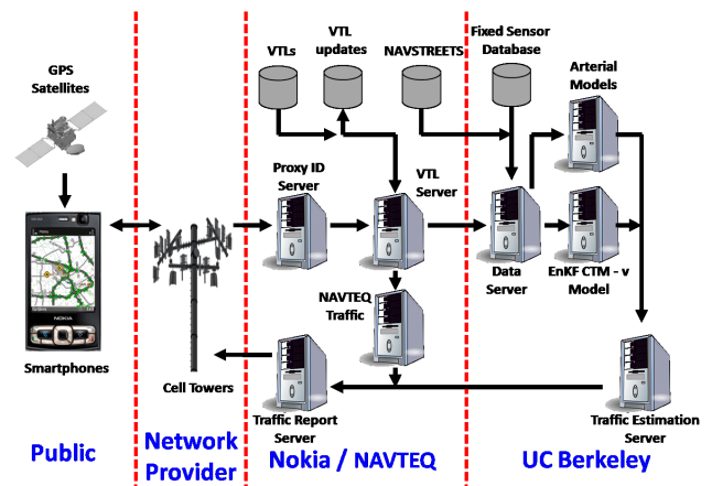
Fig. 2. System architecture overview. The system consists of vehicles equipped with GPS-enabled smartphones, a cellular network provider, an ID data collection infrastructure and traffic information provision, and traffic estimation algorithm running on the model server.
