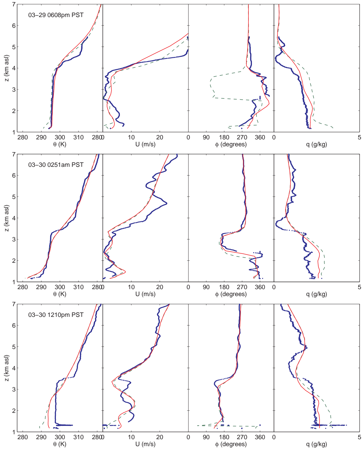
Figure 6: Selected soundings at Independence Airport of potential temperature, wind speed, wind direction, and specific humidity at 0608pm PST, 0251am PST, and 1210pm PST. — Observations; — REF; - - - SM
