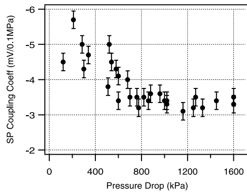
Figure 2. Relationship of C_c to pressure drop for sample Berea-2 from that time after water/CO 2 mixing was assumed to be complete, or t > 700 sec (Figure 1). Error bars reflect experimental variation due to pressure and voltage signal noise. See color version of this figure in the HTML.
