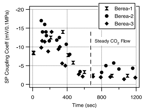
Figure 1. Coupling coefficient vs. time for samples Berea-1, Berea-2 and Berea-3. Only the initial portion of the tests are shown. The Cc was constant for times greater than 700 seconds. The size of the individual symbols approximates experimental variance. See color version of this figure in the HTML.
