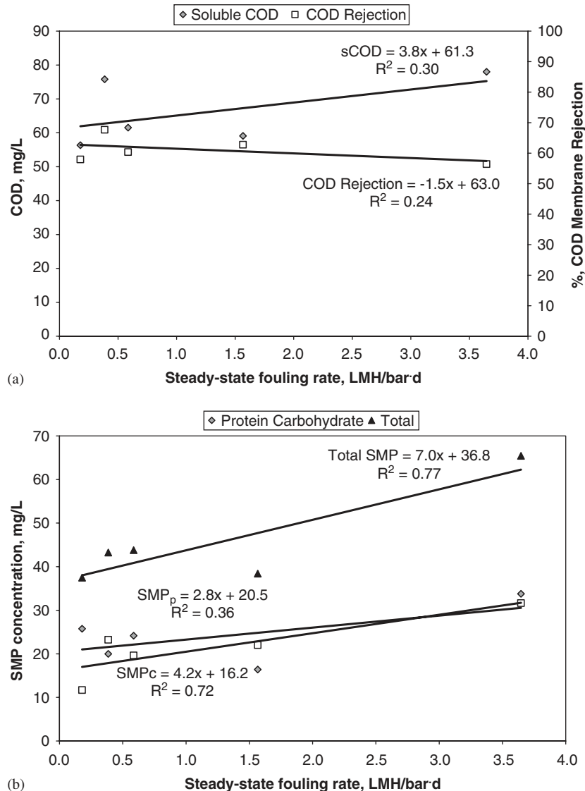
Fig. 7 – Correlations of steady-state membrane fouling rates to (a) soluble COD and COD rejection and (b) SMP_c , SMP_p , and total SMP.
