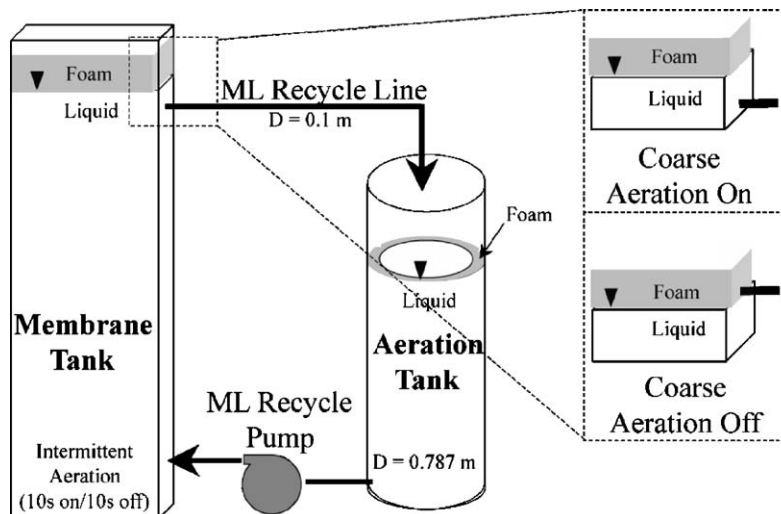
Fig. 2 – Illustration of mechanical foam control.
