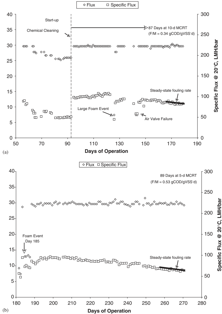
Fig. 3 – Membrane performance 10- and 5-d MCRTs.
