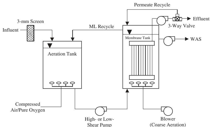
Fig. 1 – Schematic of the pilot-scale SMBR.
