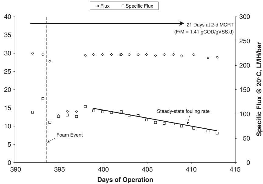
Fig. 5 – Membrane performance at 2-d MCRT.
