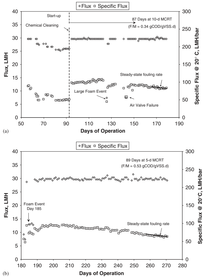
Fig. 3 – Membrane performance at (a) 10-d and (b) 5-d MCRTs.
