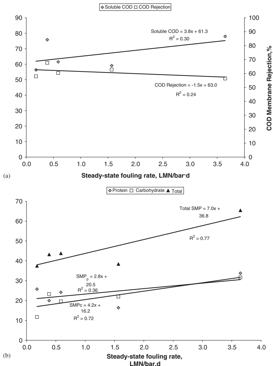
Fig. 7 – Correlations of soluble of COD and COD rejection to steady-state membrane fouling rates for the pilot-scale SMBR.
