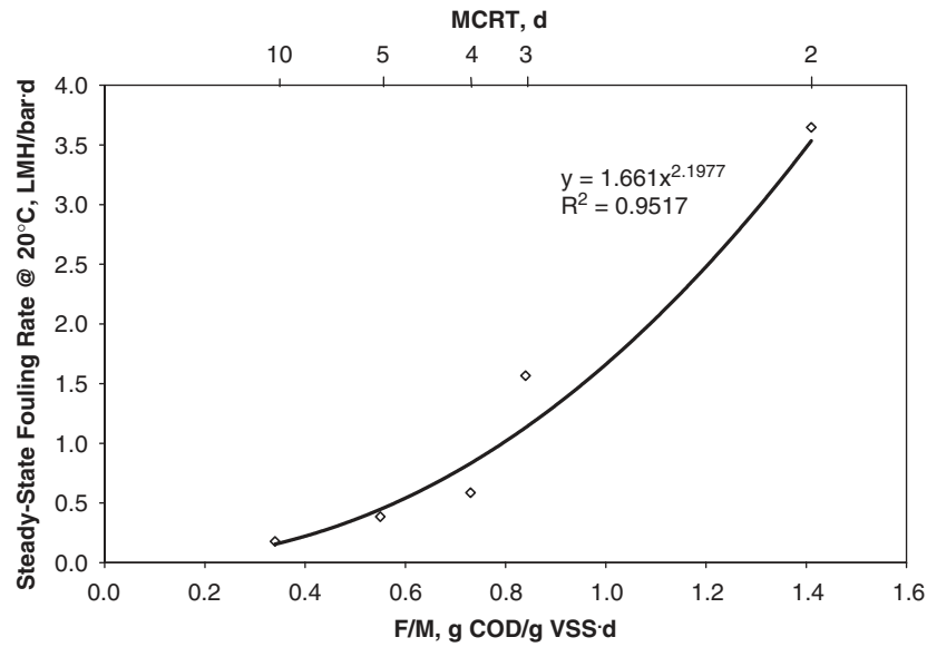
Fig. 6 – Effect of F/M on steady-state membrane fouling rate.
