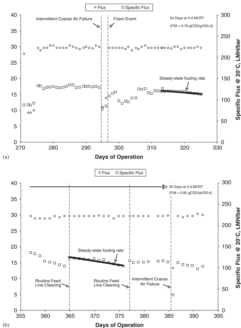
Fig. 4 – Membrane performance 4- and 3-d MCRTs.
