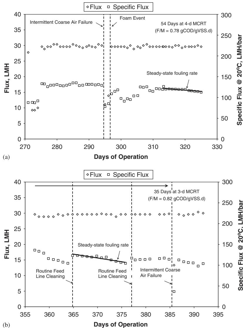
Fig. 4 – Membrane performance at (a) 4-d and (b) 3-d MCRTs.
