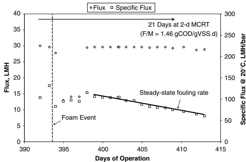
Fig. 5 – Membrane performance at 2-d MCRT.
