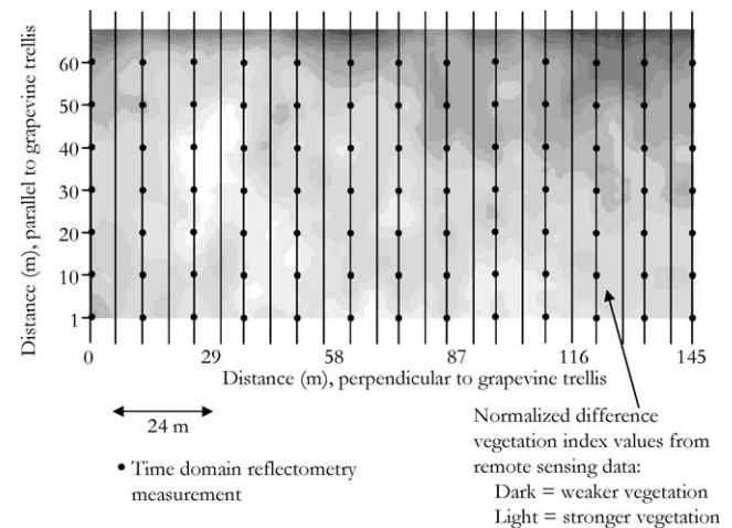
Figure 2. Site map showing GPR traverses (vertical lines) and time domain reflectometry measurement locations overlain on the normalized difference vegetation index data acquired in July 2000.
