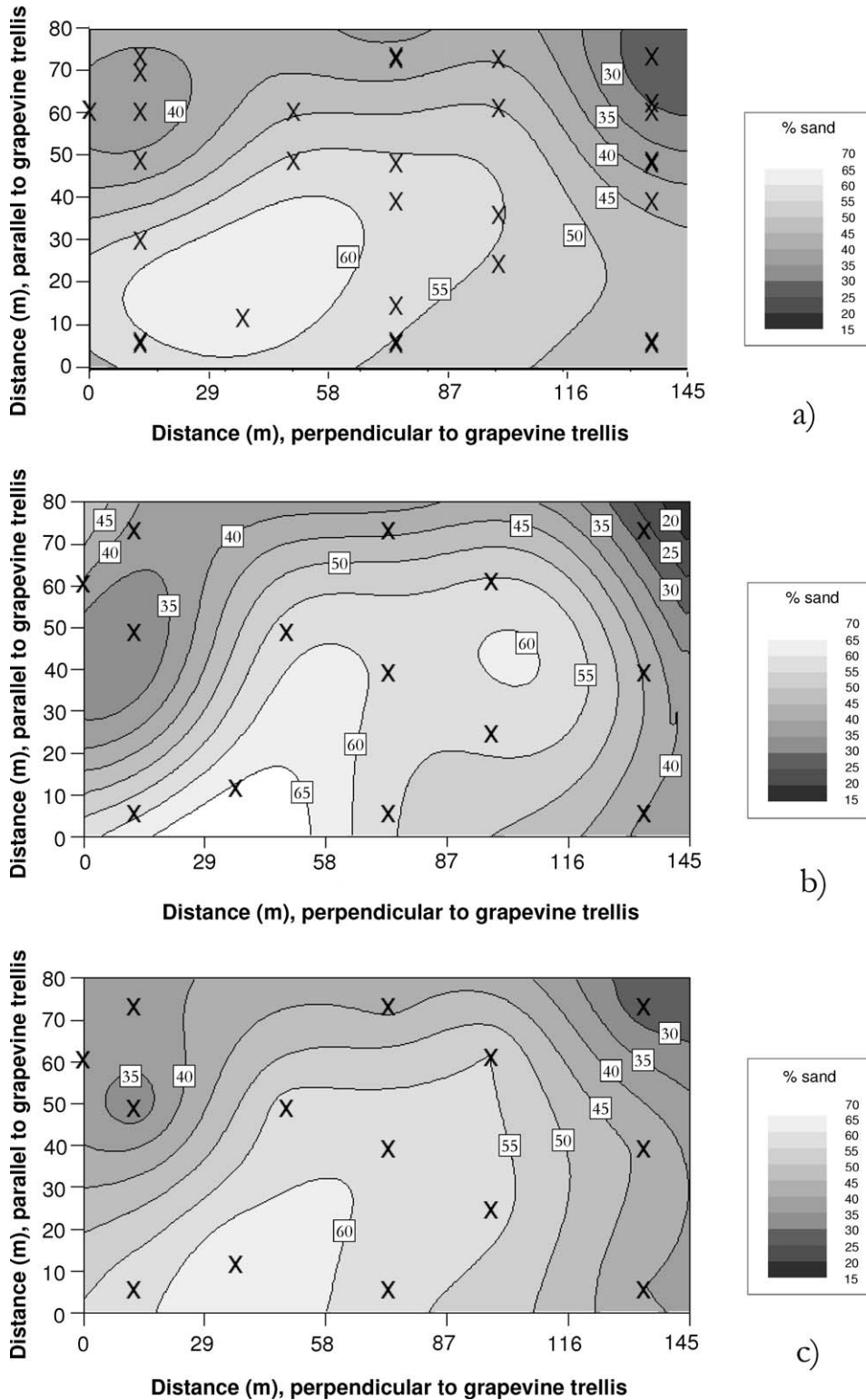
Figure 12. a) Contour map of the percent sand in the uppermost 20 cm developed using kriging of all CGSF measurements in rows without crop cover. b) Contour map of the percent sand developed using kriging of a subset of CGSF measurements in rows without crop cover. c) Contour map of the percent sand developed using co-kriging of a subset of CGSF measurements in rows without crop cover and volumetric water content estimates from 450 MHz GPR data acquired in Jan.
