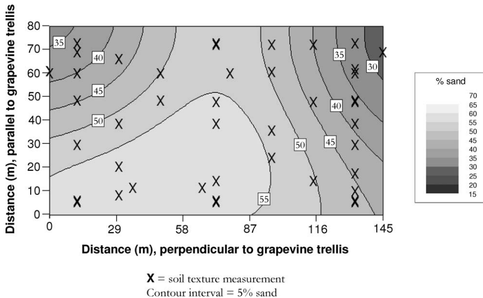
Figure 4. Contour map of soil sand fraction (% sand) in the uppermost 20 cm of the soil column across the site.
